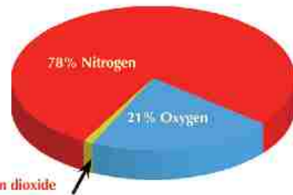
Fig (3-2): Ratios of gases in the atmosphere
